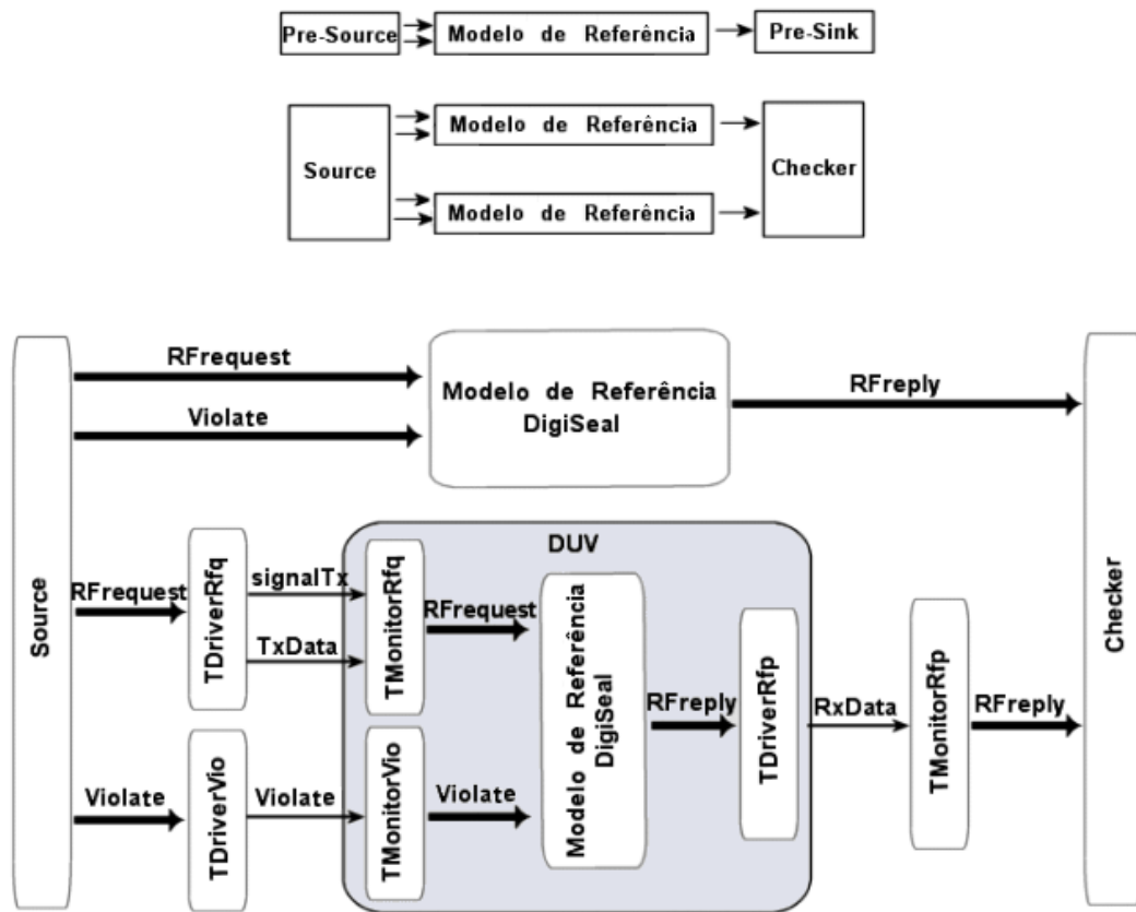
Figure 08: Testbench do DUV Completo.
