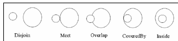
Figura 42: Predicate & Distance.
