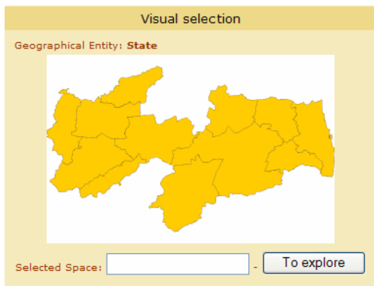
Figura 60: Visual Selection.
